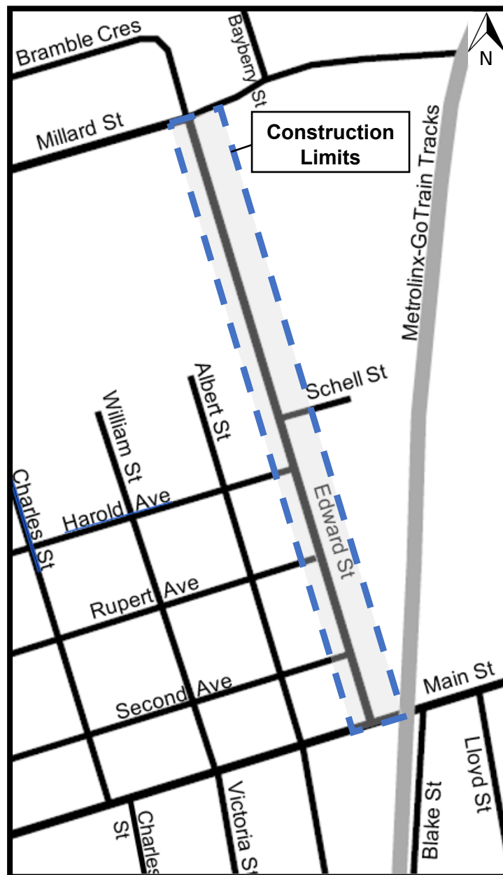
Map showing Edward Street Reconstruction limits
