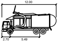
Typical Front-Load Garbage Truck
