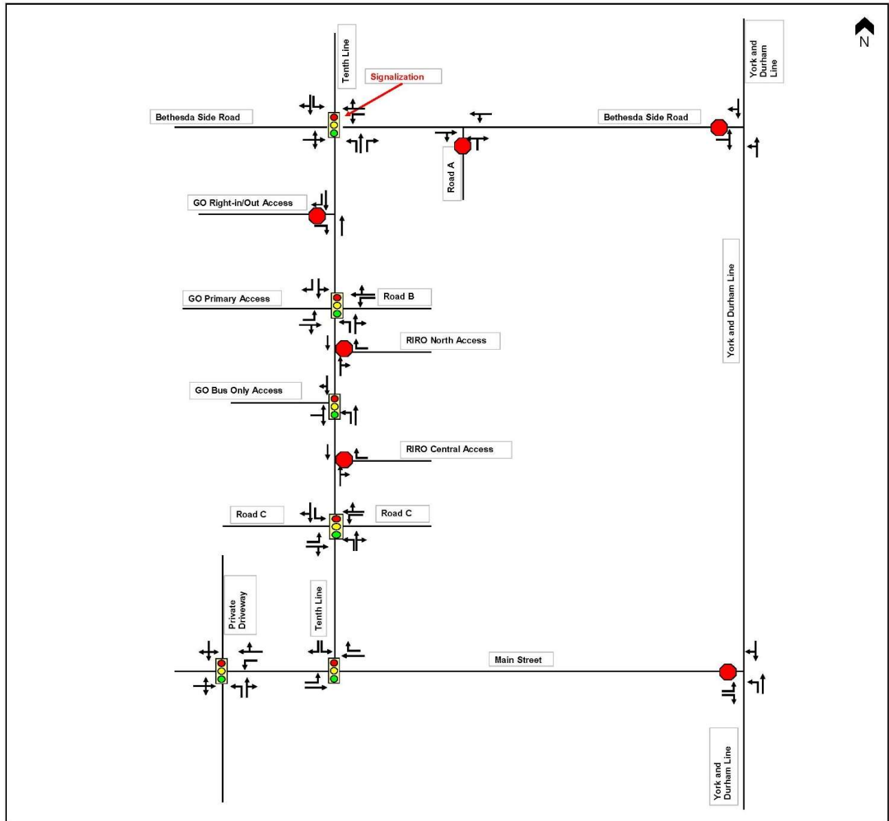
Figure 7-1 Future Total 2030 Lane Configuration
